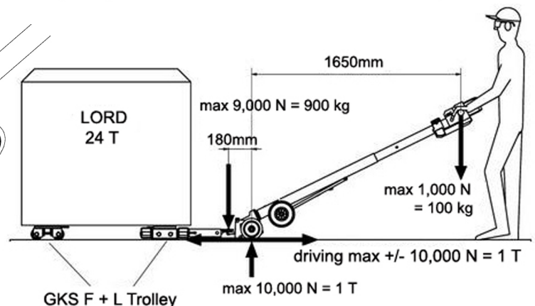
trolley adaptor
